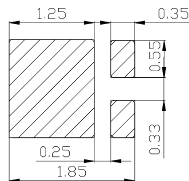
Recommended pad
